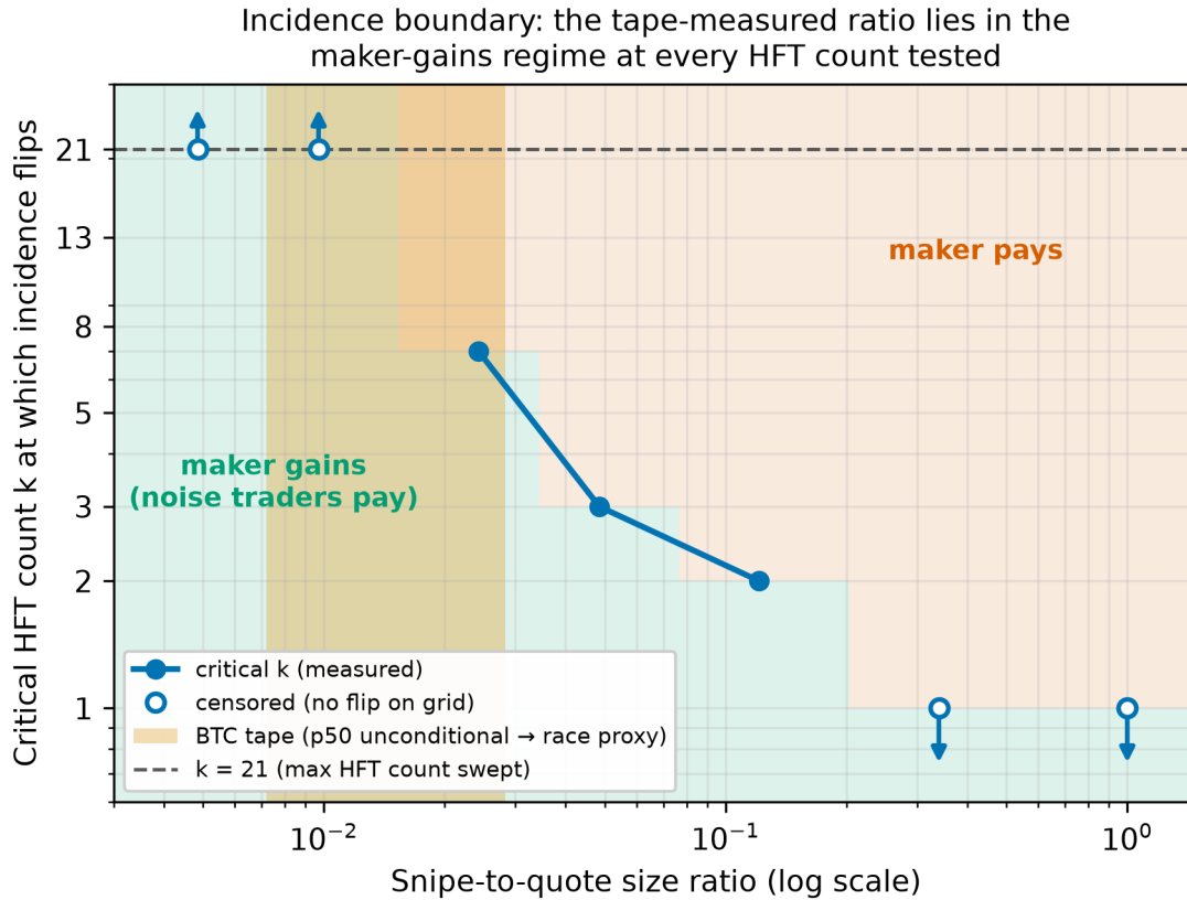
Figure 3: Incidence boundary over snipe-to-quote ratio and HFT count. The shaded vertical band is the ratio measured on the BTCUSDT-perp tape (unconditional median to race-proxy median); open markers with arrows are ratios at which no flip occurs anywhere on the swept grid.
