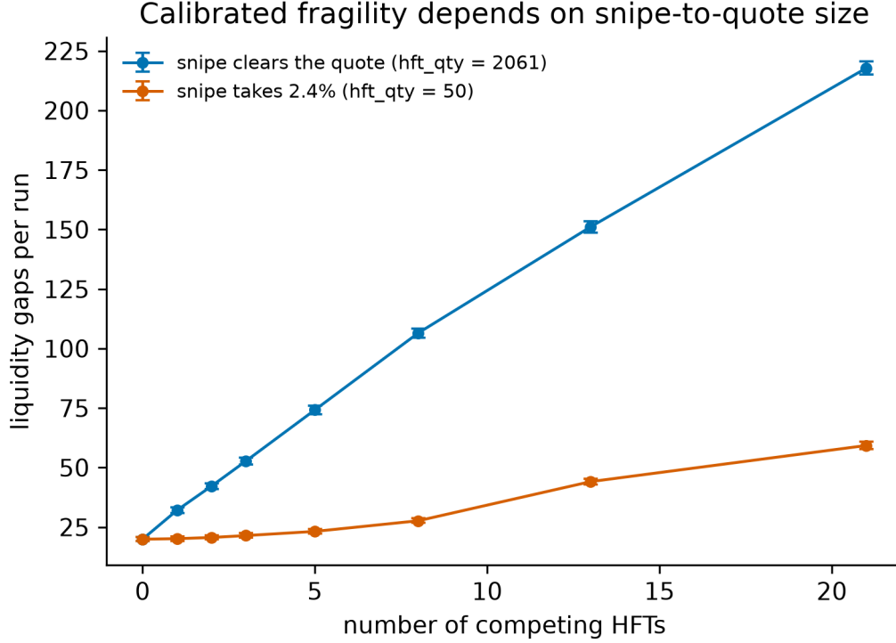
Figure 13: Liquidity gaps versus HFT count for both snipe-size arms
