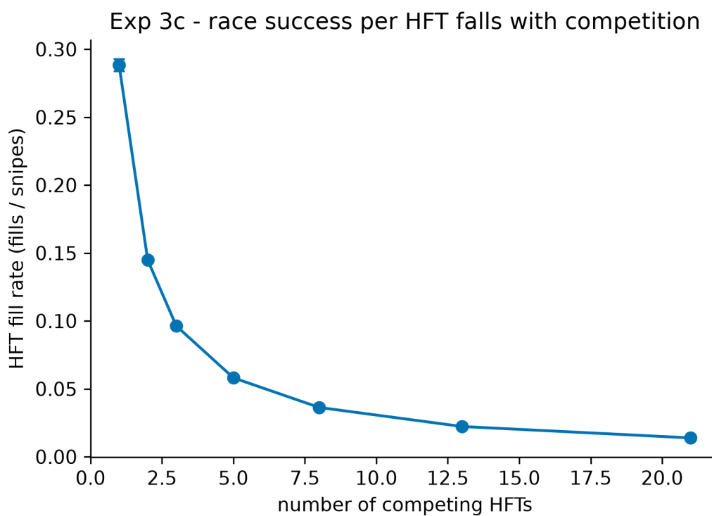
Figure 7: Per-HFT fill rate declining as 1/k
