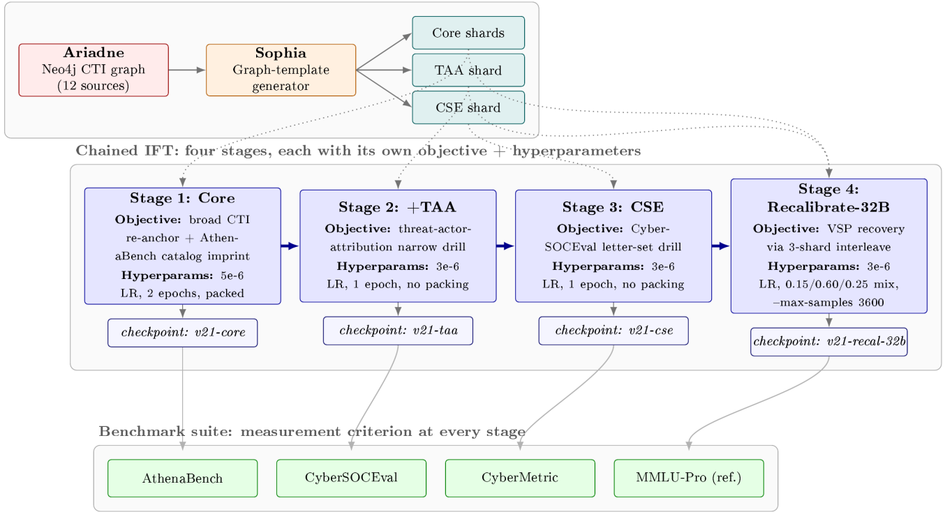
Fig. 1. The chained-IFT pattern. Sophia compiles typed graph queries against Ariadne into Alpaca-format IFT triples, sharded into Core, TAA, and CSE manifests. The four-stage chain consumes these in order: each stage has its own objective (broad CTI re-anchor for Core, narrow drills for TAA and CSE, recalibration for Stage 4) and hyperparameters. Each stage pushes a cumulative checkpoint (v21-core, v21-taa, v21-cse, v21-recal-32b), each independently evaluable against the AthenaBench / CyberSOCEval / CyberMetric / MMLU-Pro suite, supporting per-stage ablation in addition to producing a single ship checkpoint.
