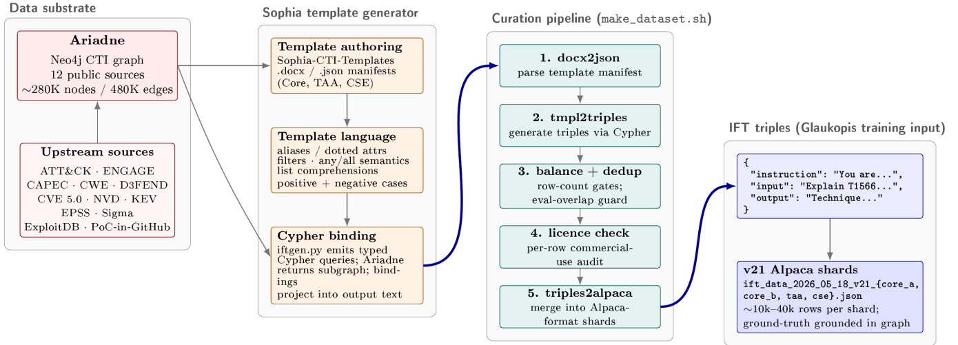
Figure 2 Sophia template generation and v21 data flow. The upstream public CTI sources (left) are ingested into the Ariadne Neo4j graph. Sophia (centre-left) authors templates in three artefacts—template manifests (.docx/.json), the template language, and the Cypher binding step in iftgen.py —each of which compiles graph queries into natural-language output. The v21 curation pipeline ( make_dataset.sh , centre-right) runs five steps in order: parse the template manifest, generate triples via Cypher, balance and dedup the corpus against the row-count gates and the eval-overlap guard (Appendix B), check per-row licence compliance, and merge the per-template files into Alpaca-format shards. The output (right) is the set of Alpaca-format IFT shard files ( ift_data_2026_05_18_v21_{core_a, core_b, taa, cse}.json ) consumed directly by the chained-IFT training stages (Section 5.4).
