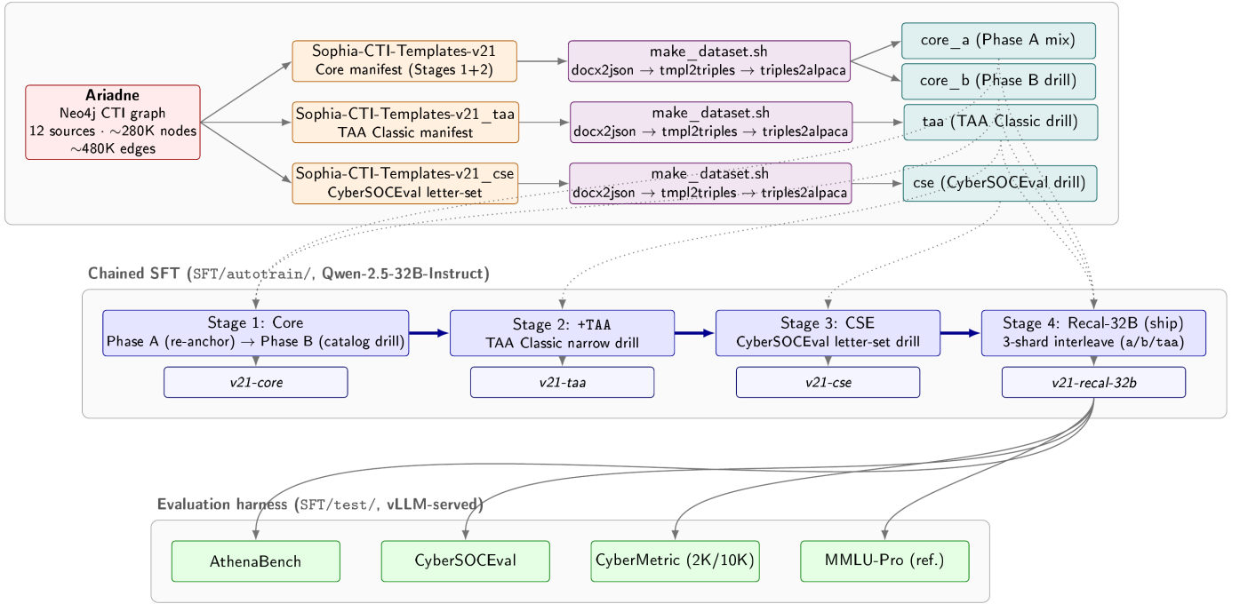
Figure 3 Glaukopis v21 end-to-end flow. Ariadne (Section 4.3), the Athena Neo4j CTI substrate, feeds three v21 template manifests—Core, TAA, and CSE—each processed by the make_dataset.sh pipeline into Alpaca-format dataset shards. Four production shards ( core_a , core_b , taa , cse ; matched validation shards omitted for clarity) drive the four-stage chained-IFT recipe targeting Qwen-2.5-32B-Instruct, producing the cumulative v21-core, v21-taa, v21-cse, and ship v21-recal-32b checkpoints. Dotted arrows mark which shards feed which stages; Stage 4 re-uses Core-A, Core-B, and TAA as a three-shard interleaved touch-up. Each pushed checkpoint is evaluated against the AthenaBench, CyberSOCEval, CyberMetric, and MMLU-Pro suites under a vLLM-served harness.
