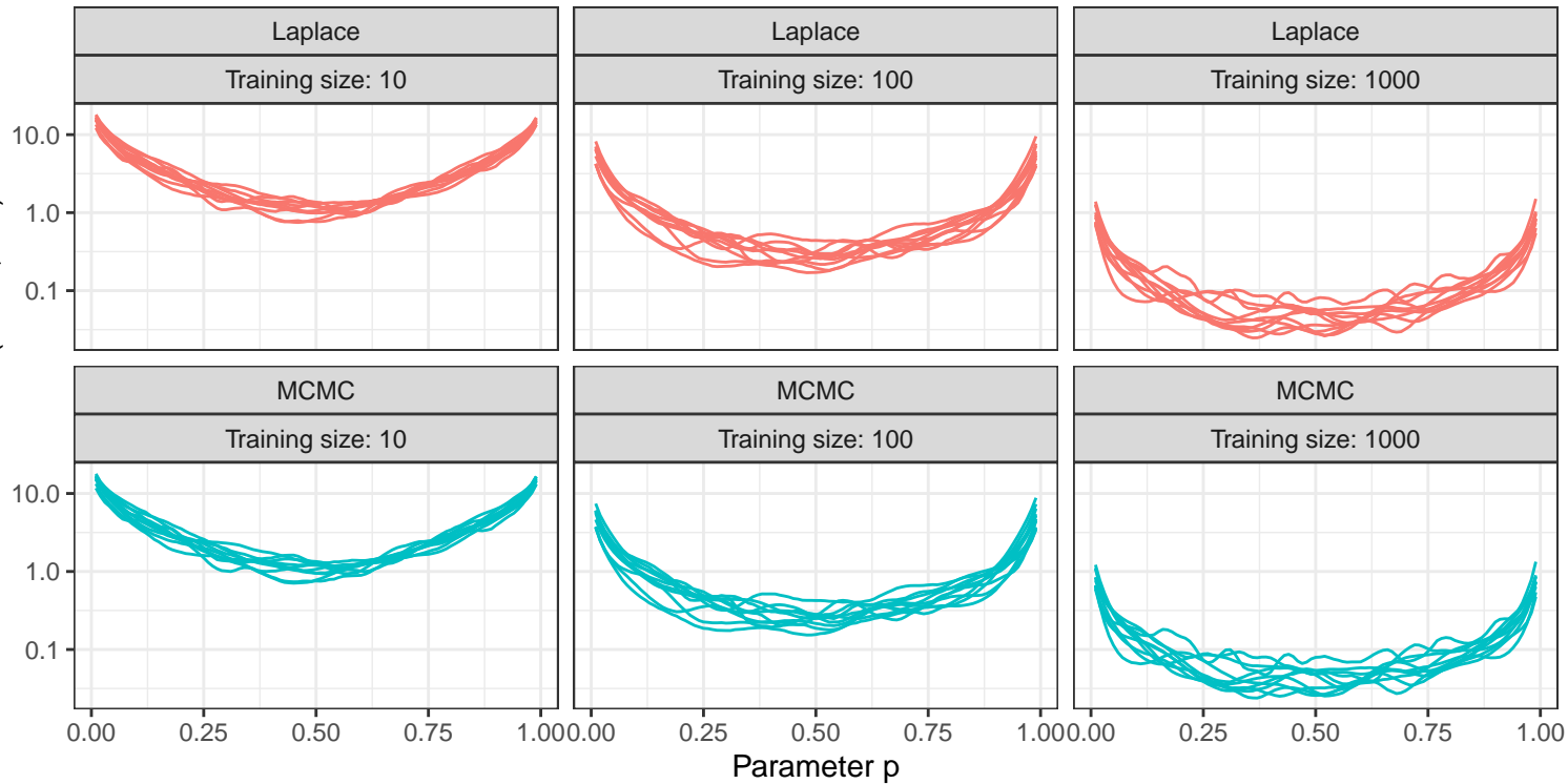
Median value of KL(SLGP, Bin)
