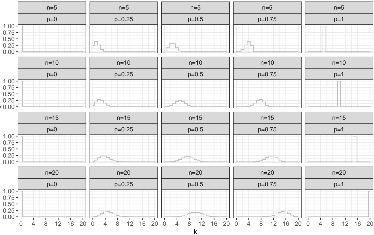
Probability
