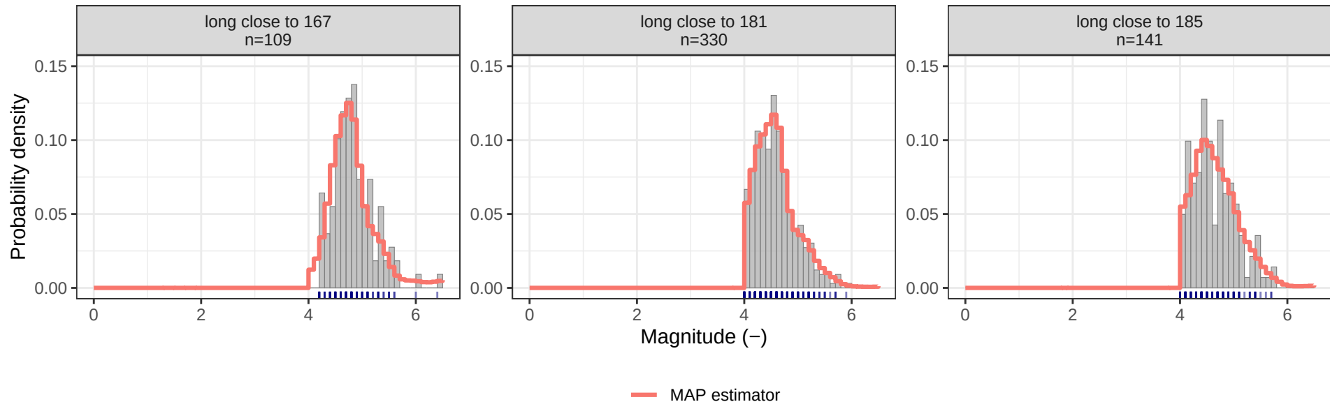
Binned 'mag' histograms by 'long' (width = 2) VS SLGP-MAP estimators at bins centers
