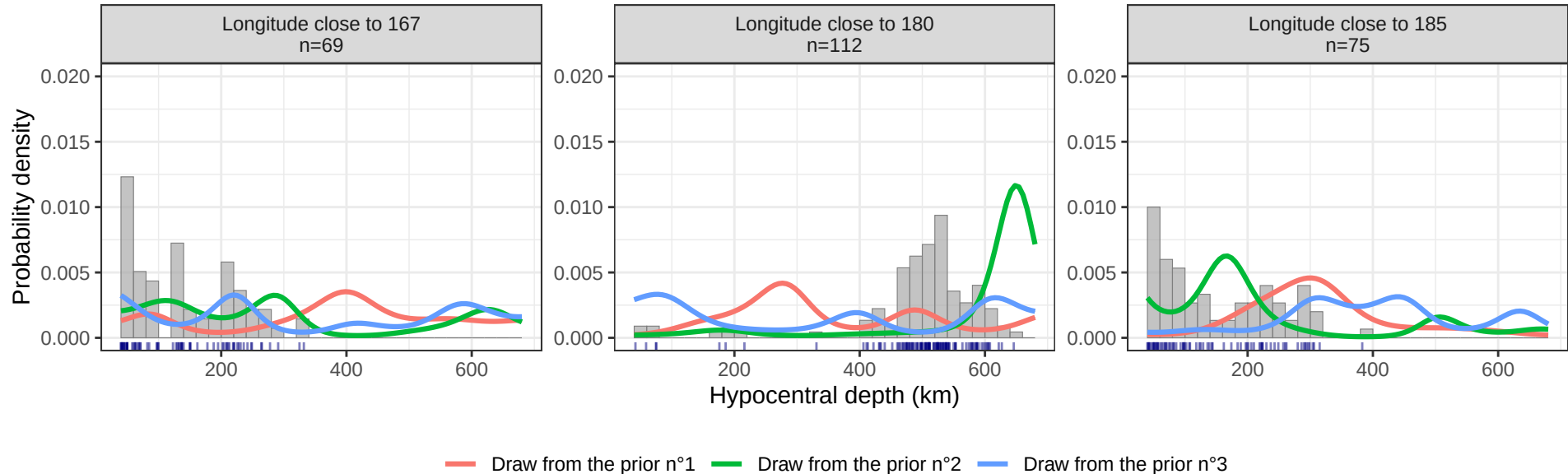
Binned 'depth' histograms by 'long' (width = 1) VS three SLGP prior draws at bins centers
