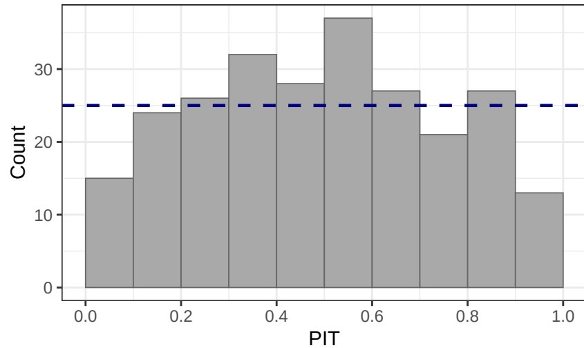
PIT histogram
