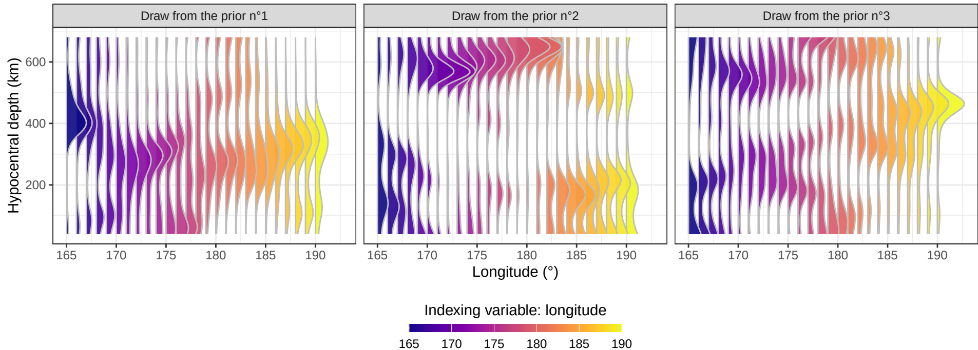
Prior SLGP samples of conditional depth densities, visualised across slices
