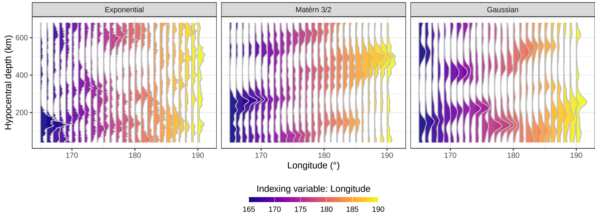
Prior SLGP samples, visualised across slices. SLGPs have varying degrees of smoothness.
