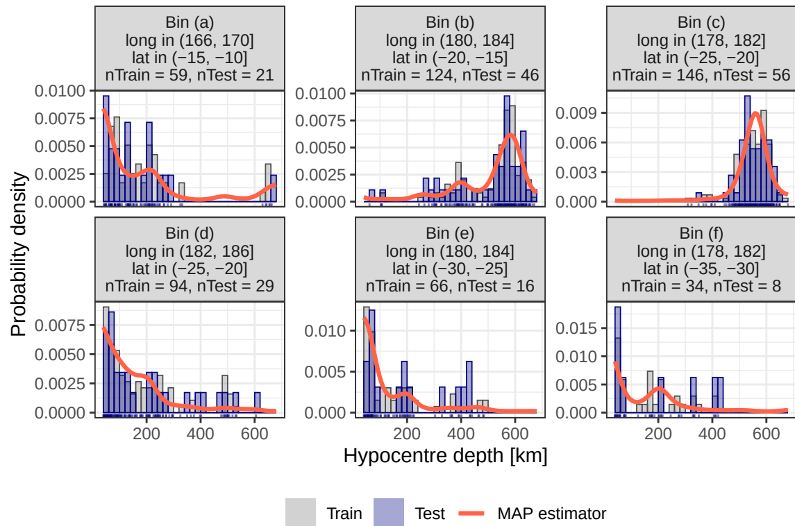
Empirical depth distributions vs SLGP estimates at bin centres
