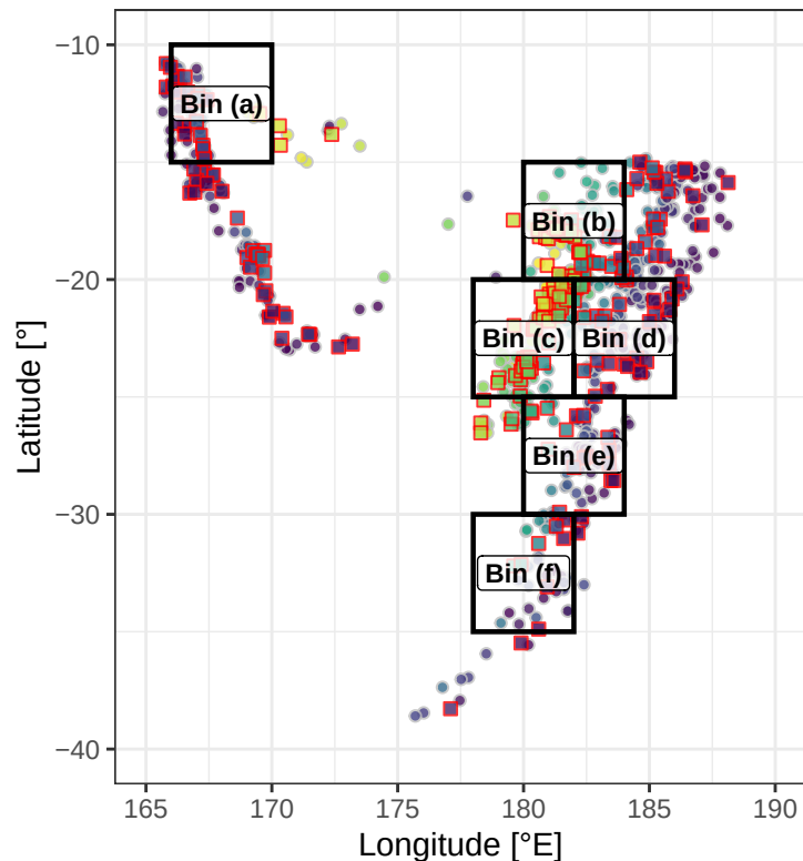
Observed hypocentre depths
