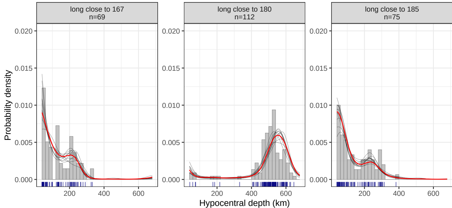
Binned 'depth' histograms by 'long' (width = 1) VS SLGP-MCMC estimators at bins centers
