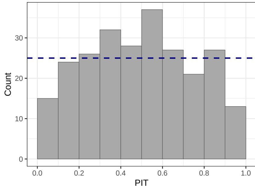
PIT histogram
