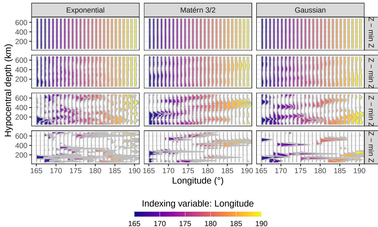
Prior SLGP samples of conditional depth densities, visualised across slices SLGPs have varying degrees of smoothness
