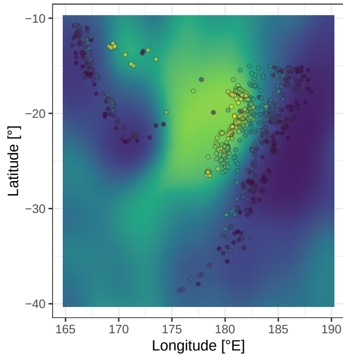
Conditional mean
