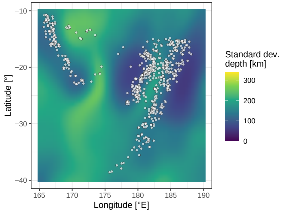
Conditional standard deviation
