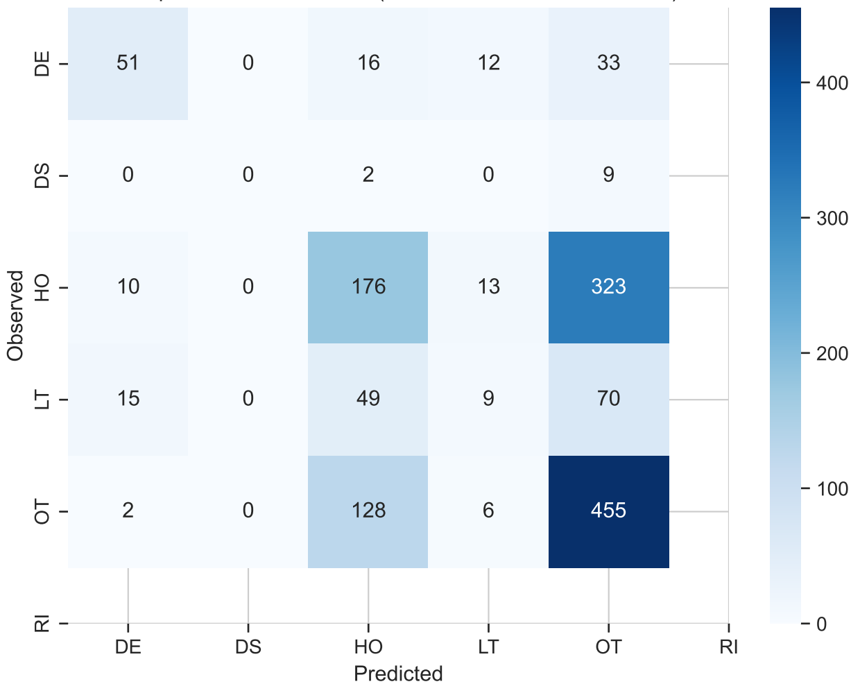
Temporal Confusion Matrix (2025 Observed-Label Test Set)
