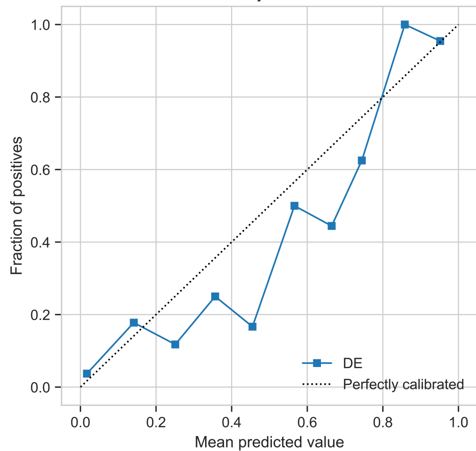
Reliability Curve: LT
