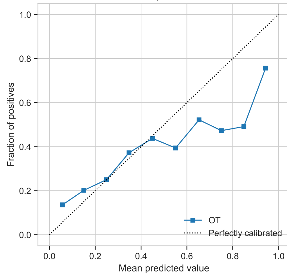
Reliability Curve: OT
