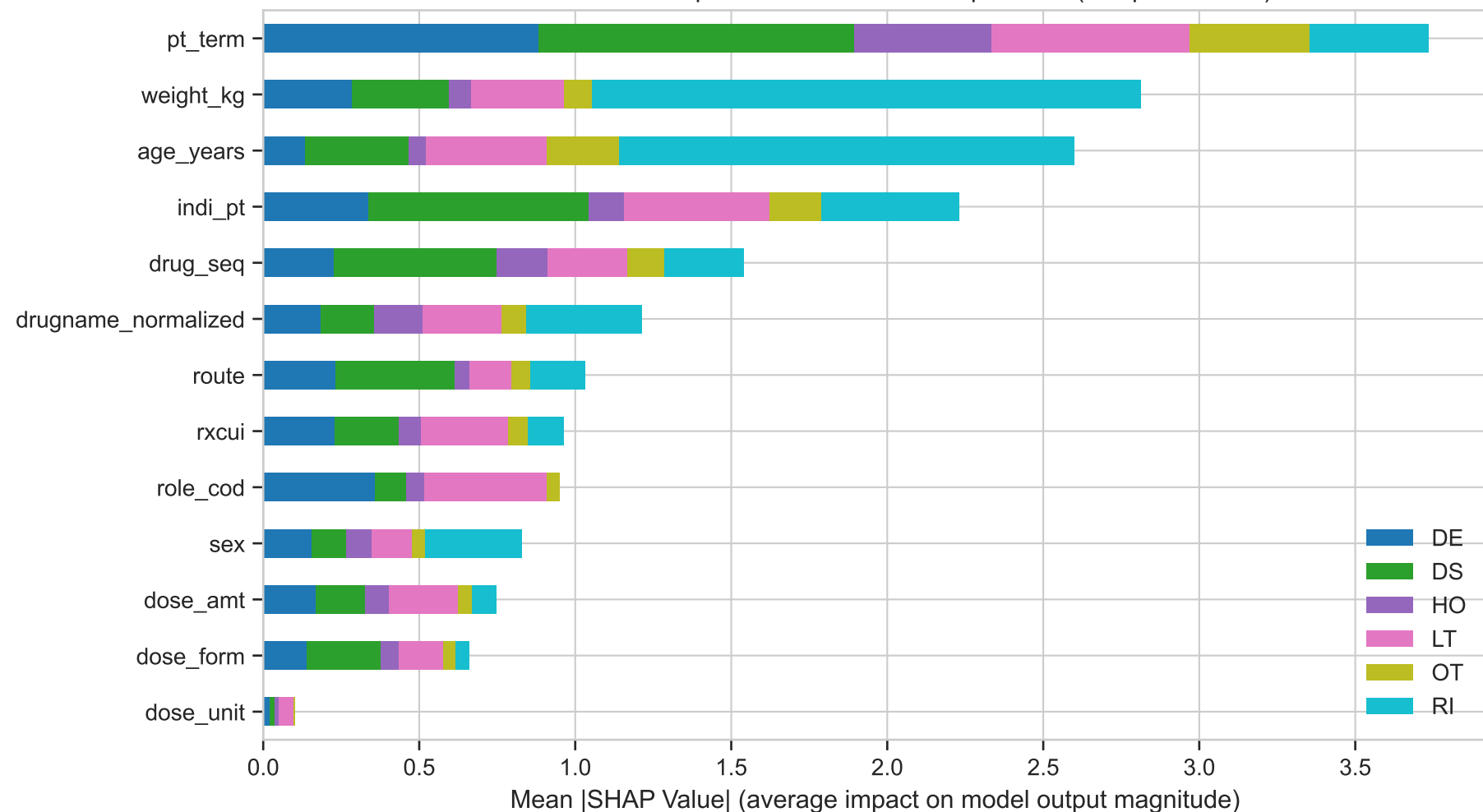
Global and Class-Specific SHAP Feature Importance (Temporal Model)
