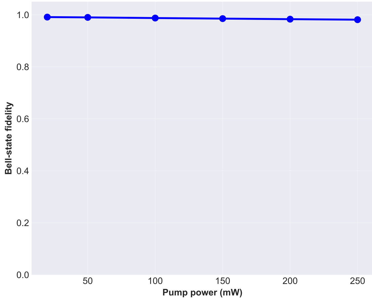
Fig 2C (right): Bell fidelity vs pump power
