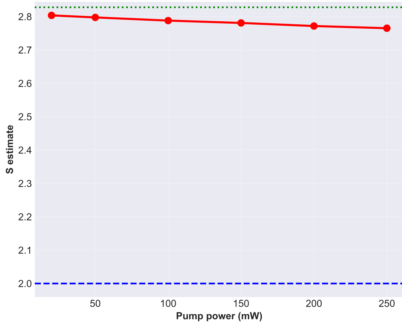
Fig 2C (left): S estimate vs pump power
