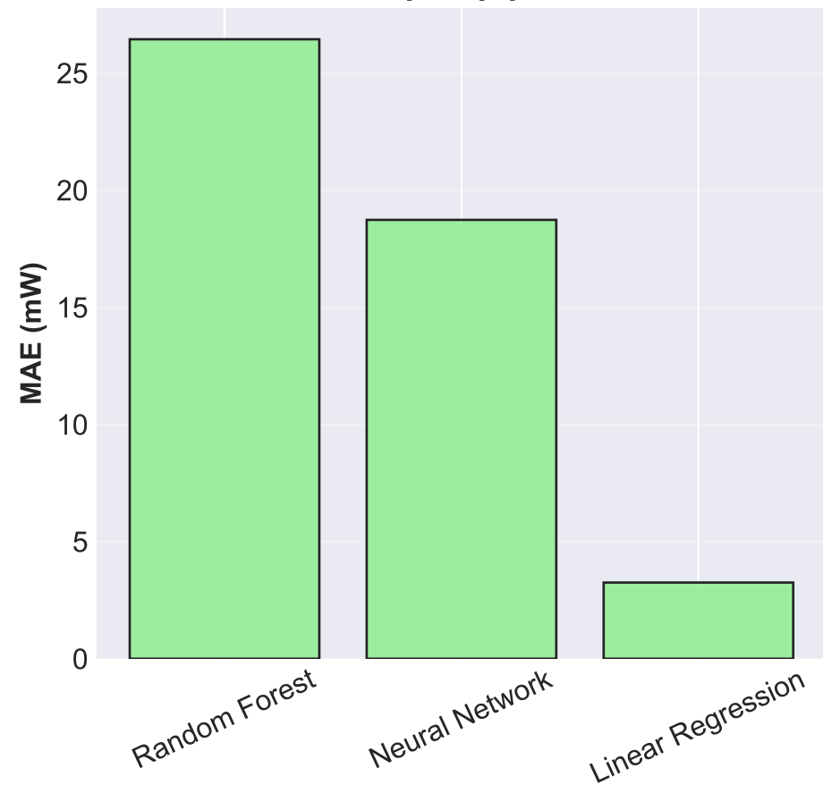
MAE when each pump power is held out
