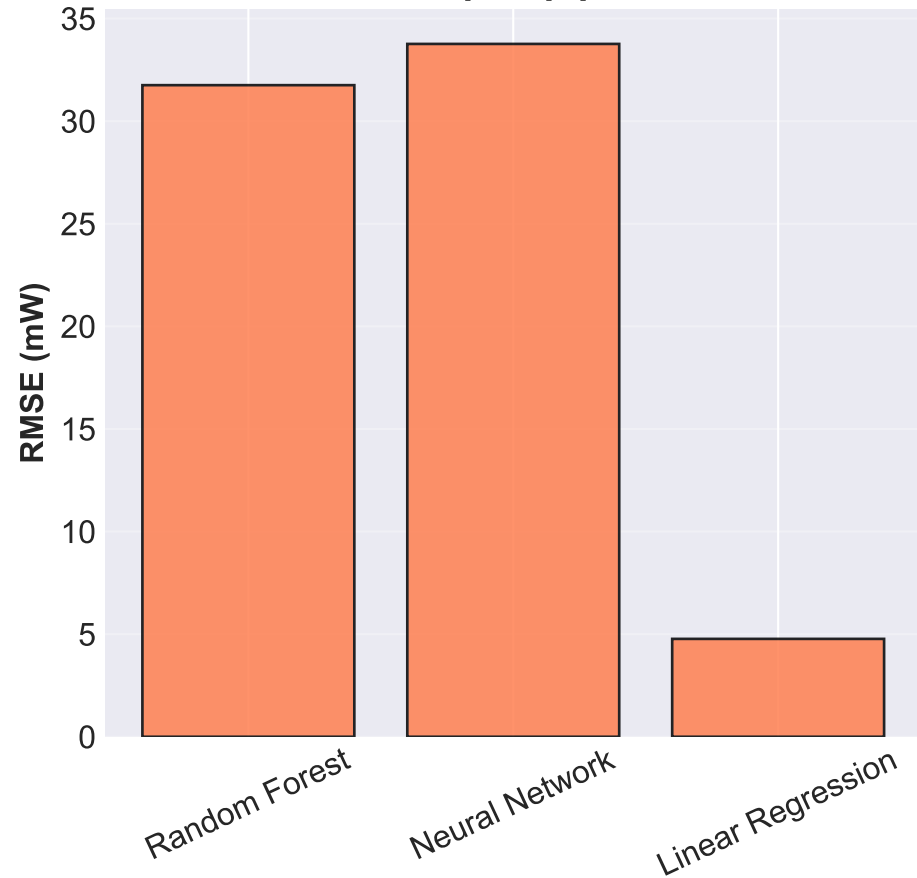
RMSE when each pump power is held out
