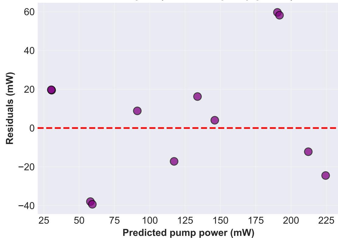
Residual plot (leave-one pump power)
