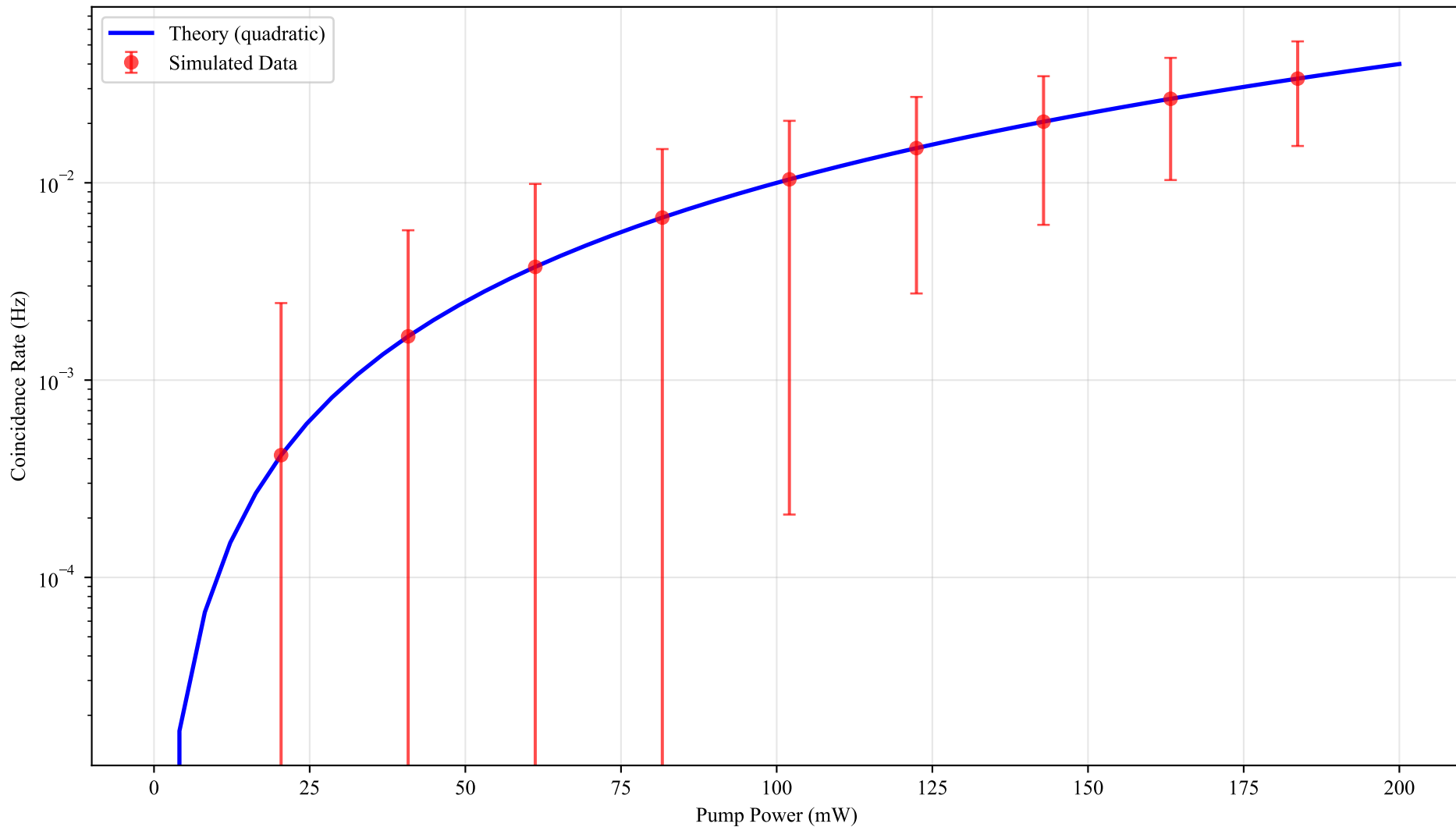
SPDC Coincidence Rate: Theory vs Simulated Experiment
