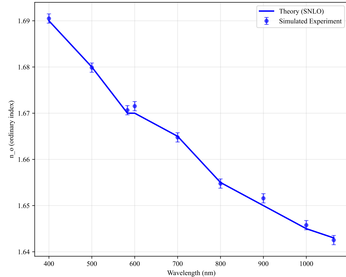
(a) Ordinary Refractive Index: Theory vs Experiment
