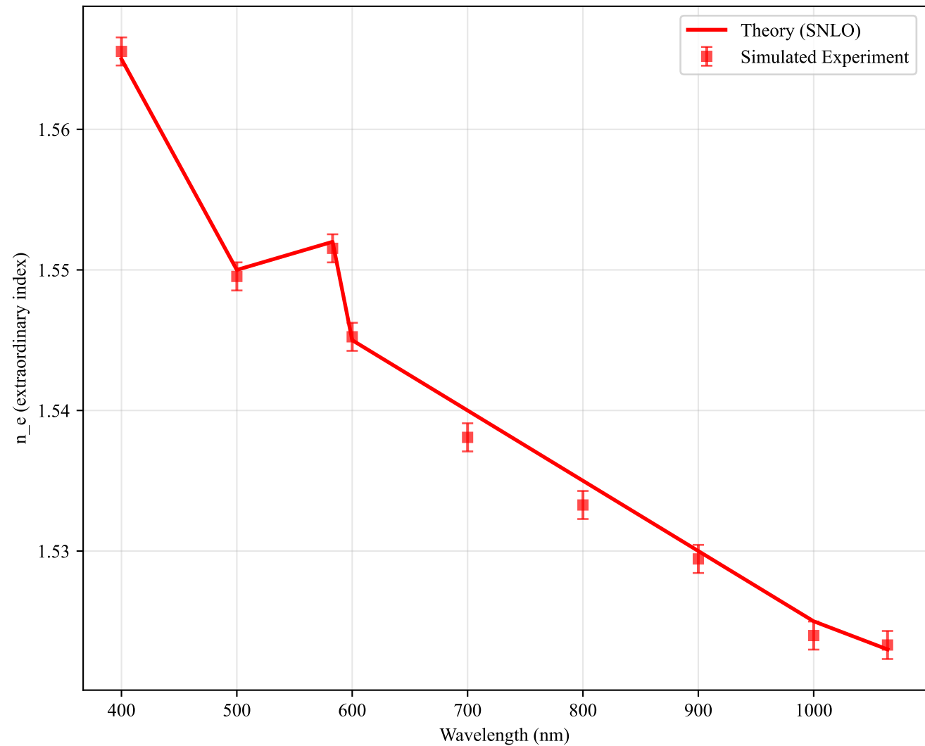
(b) Extraordinary Refractive Index: Theory vs Experiment
