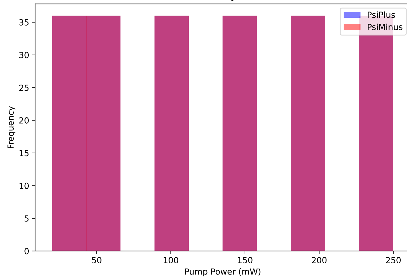
Power Distribution by Quantum State
