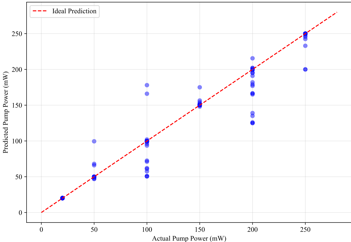
SPDC Power Prediction from Coincidence Counts ( R^2 = 0.925 , RMSE = 22.0 mW)
