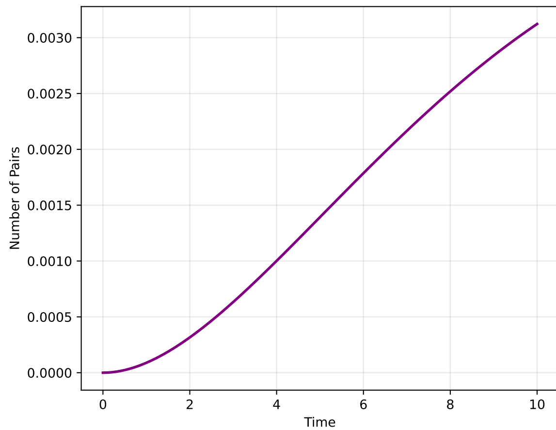
Signal-Idler Correlation
