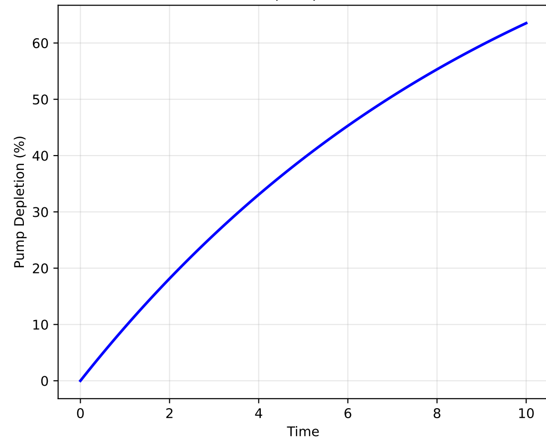
Pump Depletion
