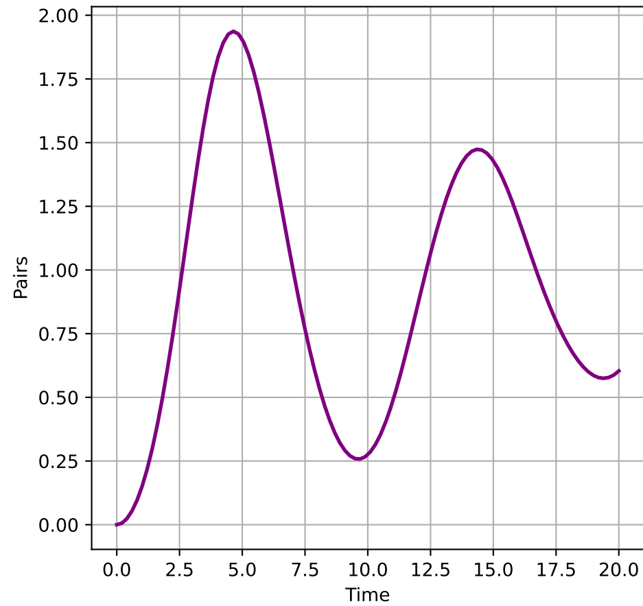
(e) Entanglement Measures
