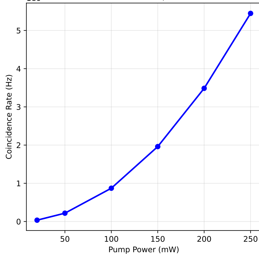
(e) Rate vs Pump Power
