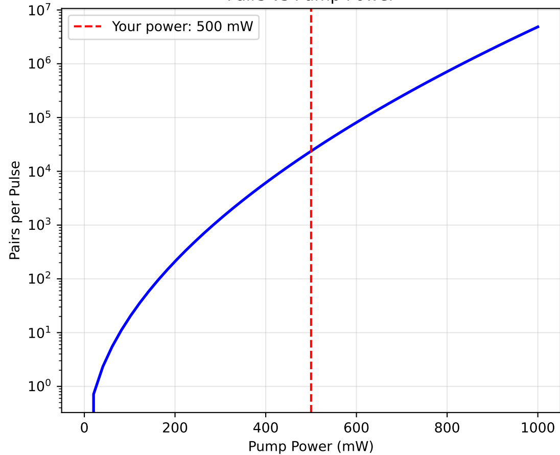
Pairs vs Pump Power
