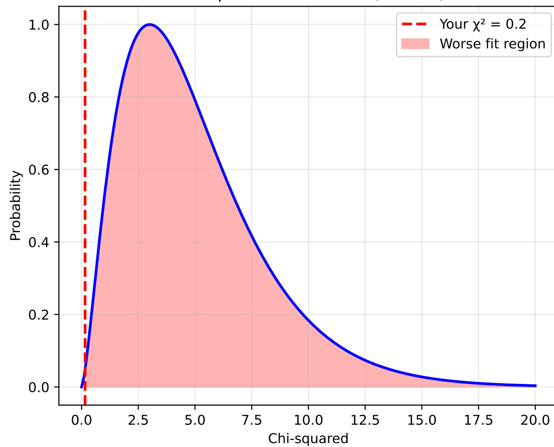
Chi-squared Distribution (dof = 5)
