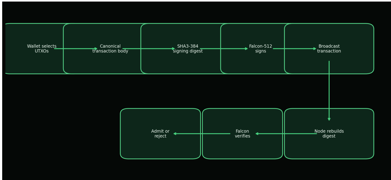
Figure 3. Transaction signing and verification bind wallet-created transaction bytes to the ATHO_TX_SIGN_V1 domain and the SHA3-384 signing digest.
