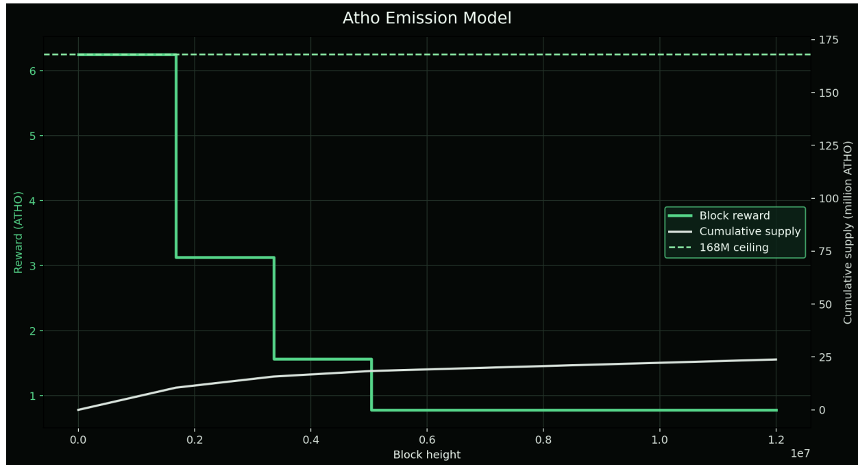
Figure 6. Emission schedule derived from the current source constants: 6.25 ATHO initial subsidy, 1,680,000-block halving intervals, and a permanent 0.78125 ATHO tail reward.
