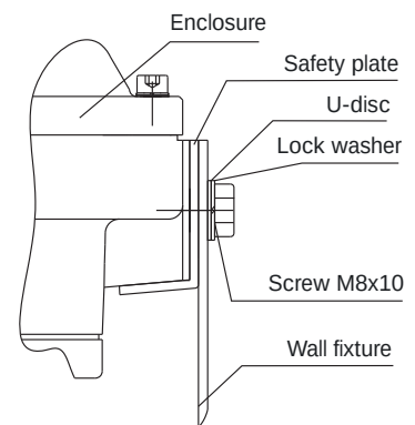
Mounting Wall Fixture
