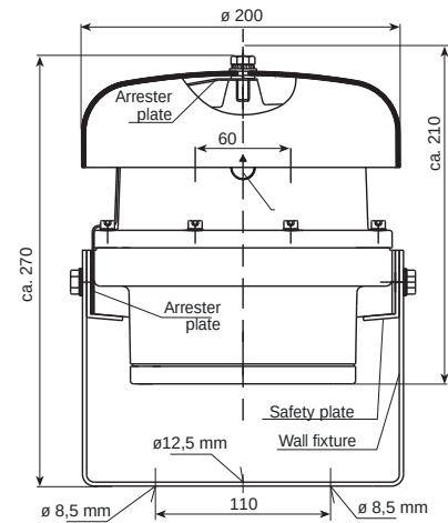
General arrangement all dimensions in mm
