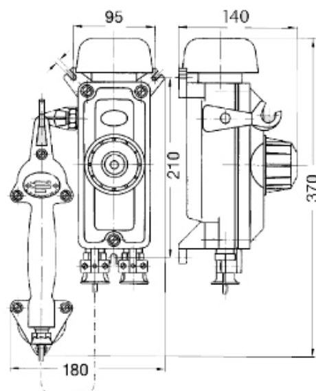
General arrangement (all dimensions in mm )
