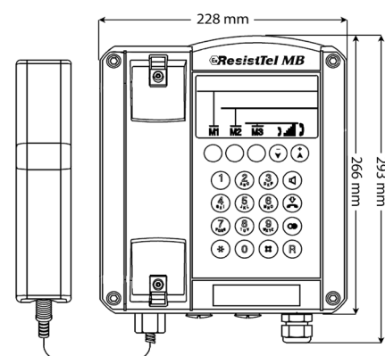
General arrangement (all dimensions in mm)
