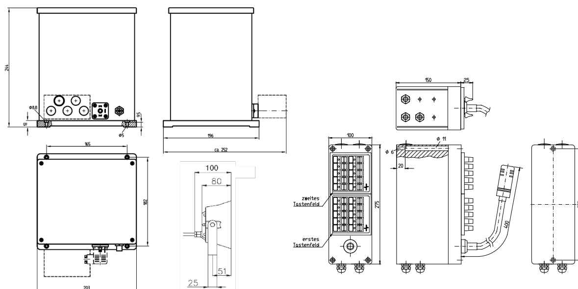
Figure: Dimensional drawing 20 / 32 FKUD .. or 20 / 32 FKVD
