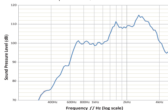
DB20 IIB, 8W, 1m SPL vs Frequency Swept sine wave, unsmoothed ±3dB
