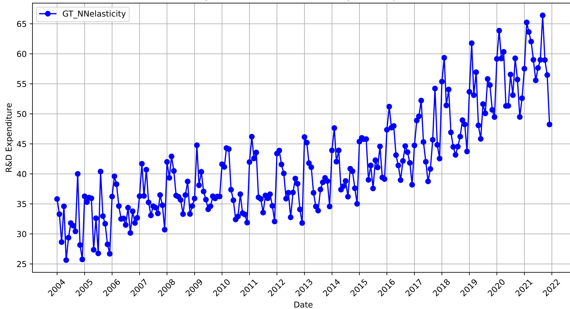
NN-driven Elasticity-based Estimates for Monthly R&D Expenditures in the US
