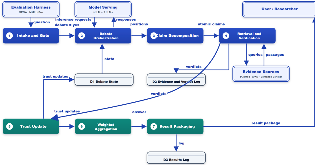
Figure 3.2: Level-one data flow diagram of the trust-calibrated multi-agent deliberation framework.
