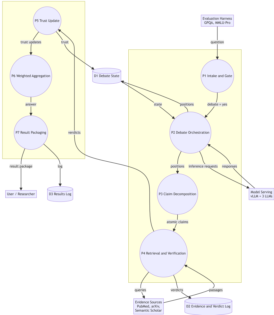
Figure 3.2: Level-one data flow diagram of the trust-calibrated multi-agent deliberation framework.
