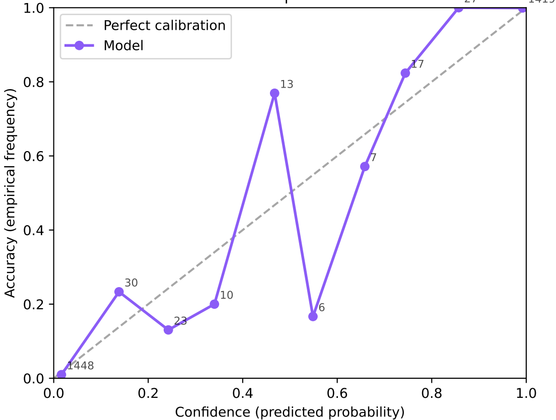
Reliability diagram ECE=0.0128 | Brier=0.0116
