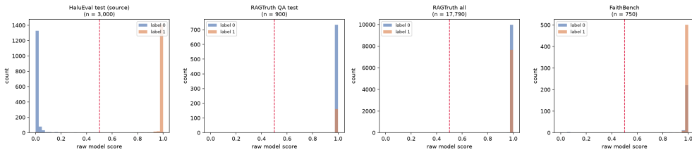
Figure 6: Raw model score distributions on the HaluEval test set and the zero-shot corpora, with the 0.5 threshold marked. The source panel separates the classes, while every zero-shot panel piles both labels at 1.0.
