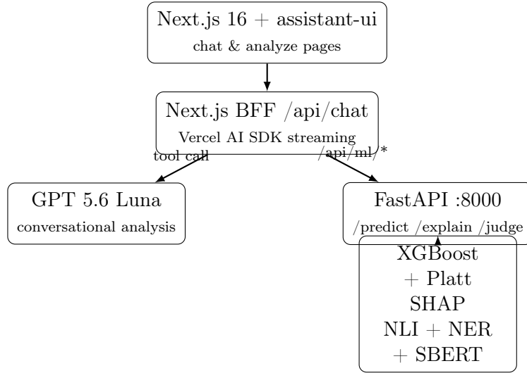
Figure 4: HaluRISC system architecture: the Next.js backend-for-frontend proxies ML requests to FastAPI and streams LLM chat with tool-generated UI widgets.
