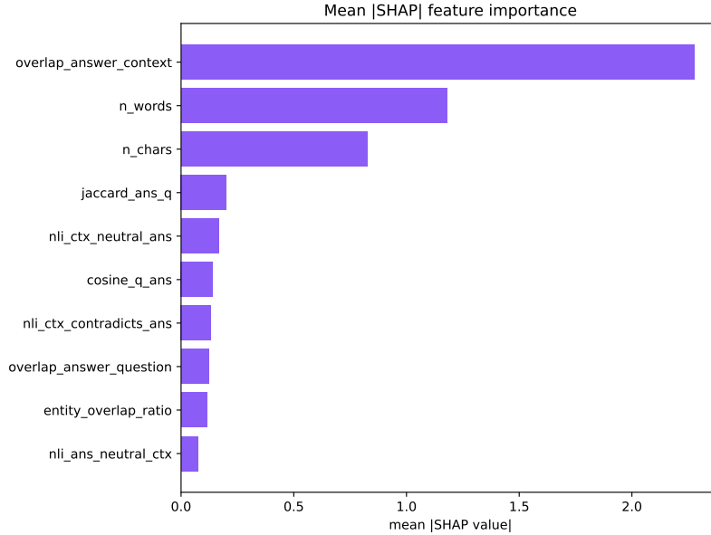
Figure 6: Mean |SHAP| feature importance (top 10).
