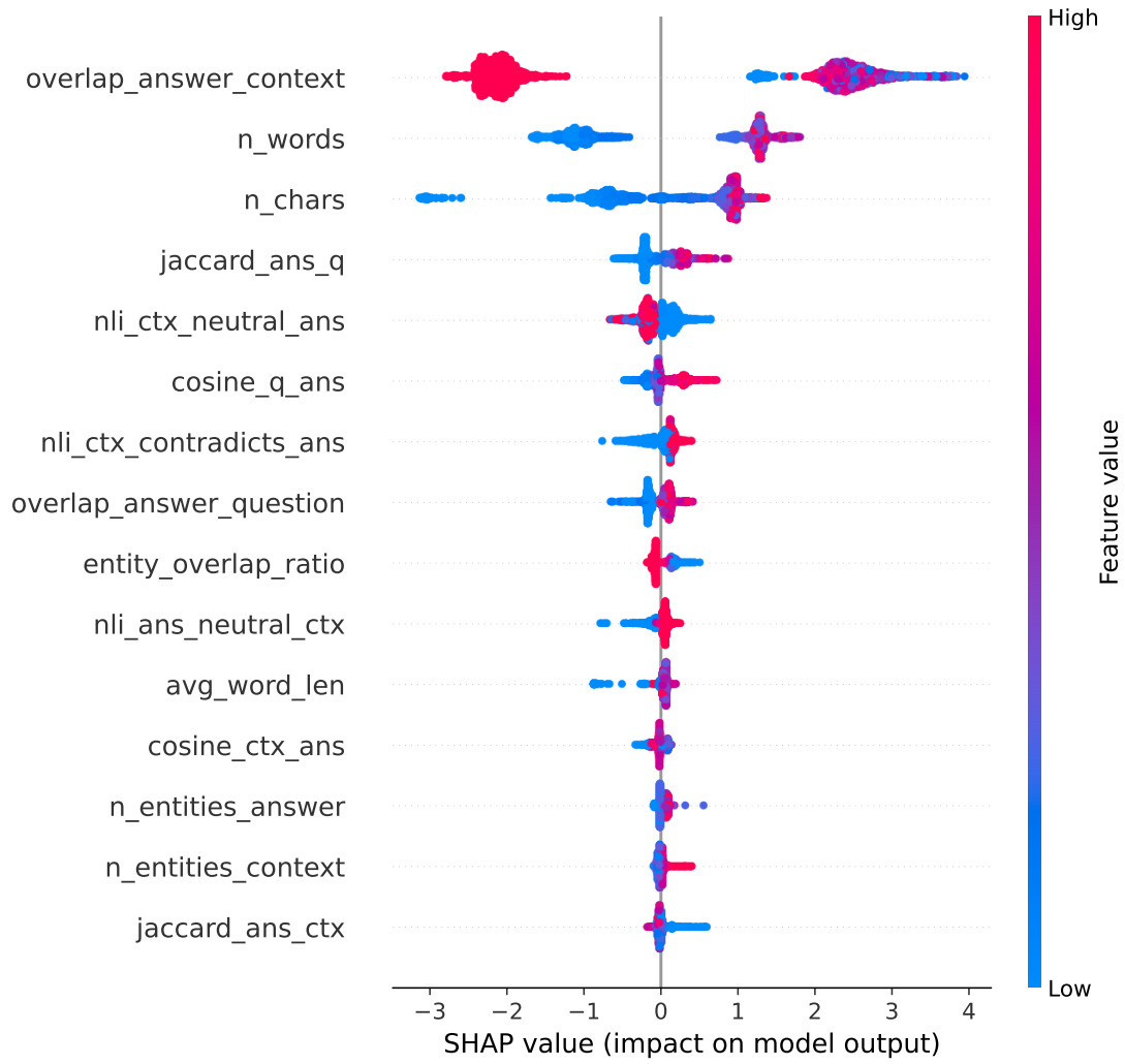
Figure 7: SHAP beeswarm summary over the test set.
