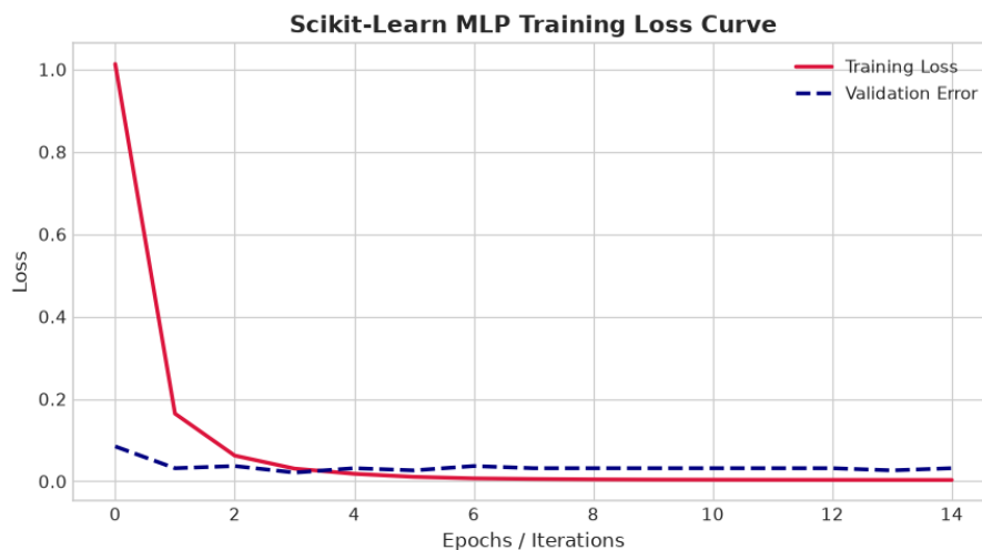
Figure 13.1: Training loss curve of the scikit-learn MLP; early stopping halted training after 15 iterations.
