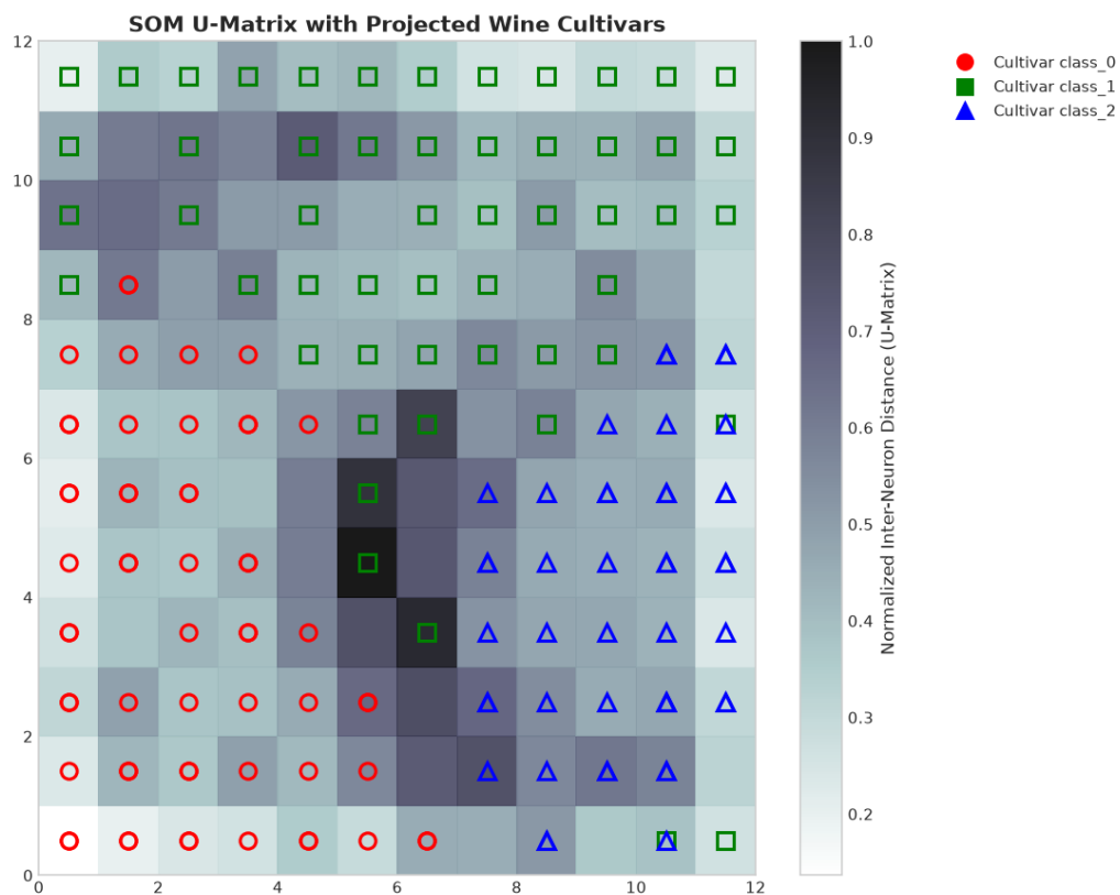
Figure 15.1: SOM U-matrix with the wine samples projected onto their BMUs; marker shape and color encode the true cultivar.
