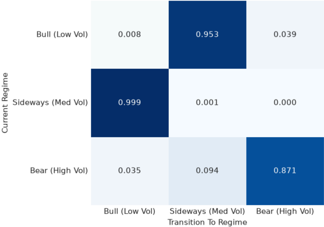
HMM Transition Probability Matrix ( A_{ij} )
