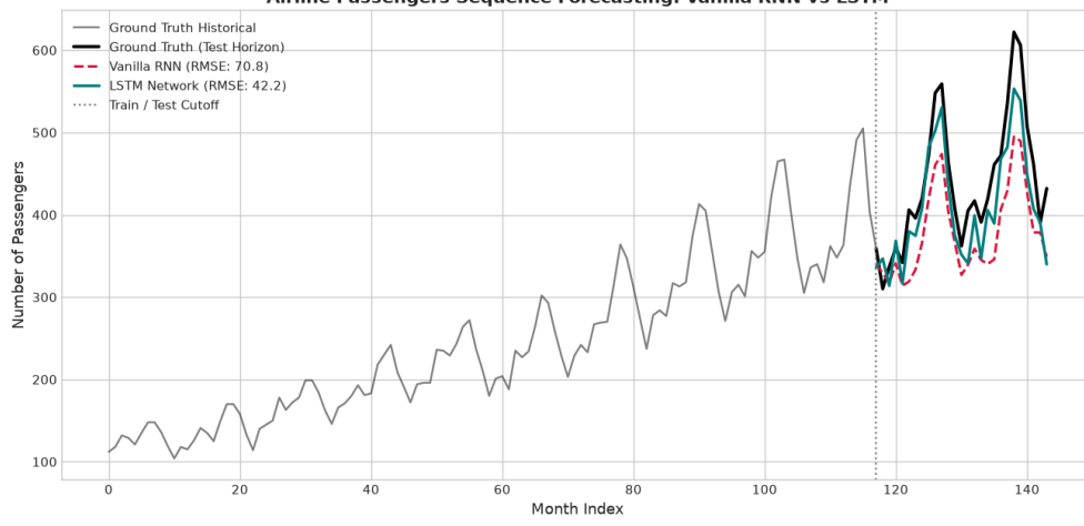
Airline Passengers Sequence Forecasting: Vanilla RNN vs LSTM
