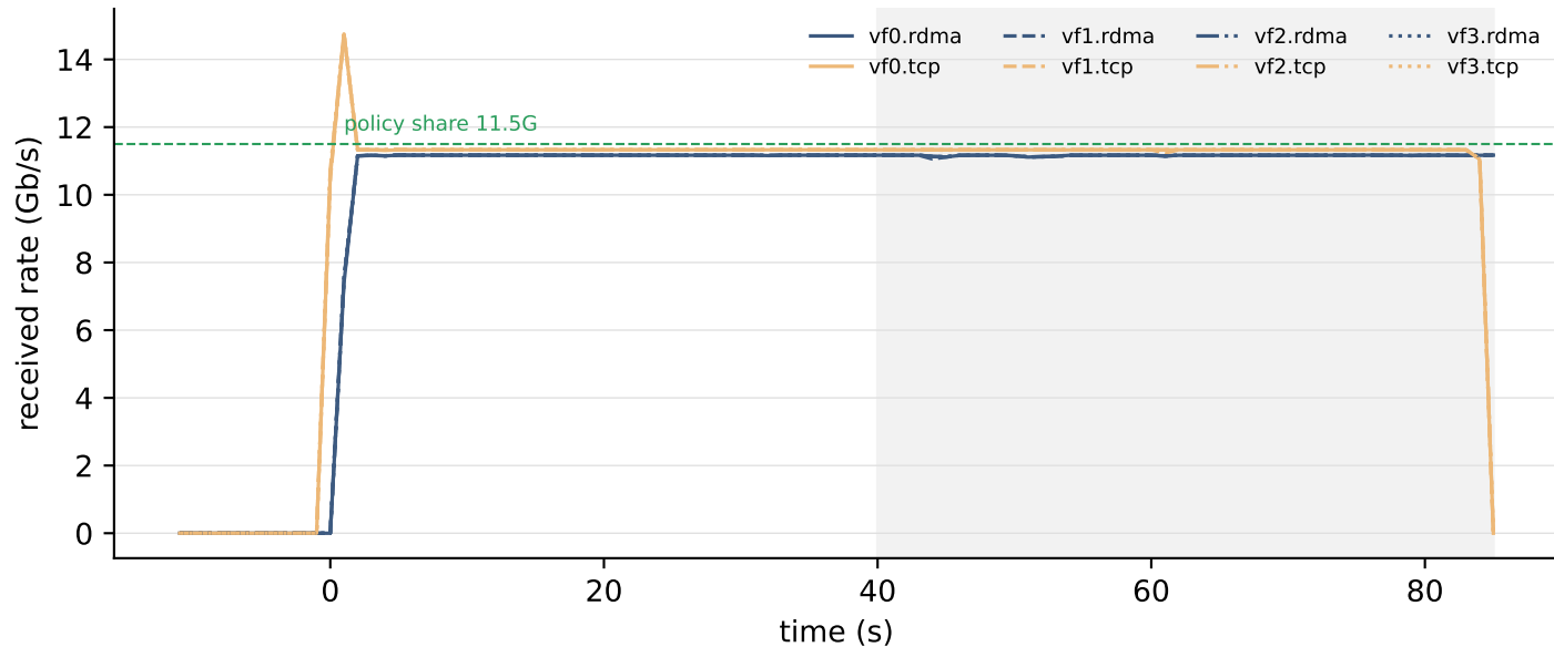
incast8 — DCQCN, coupled recovery, run 1
