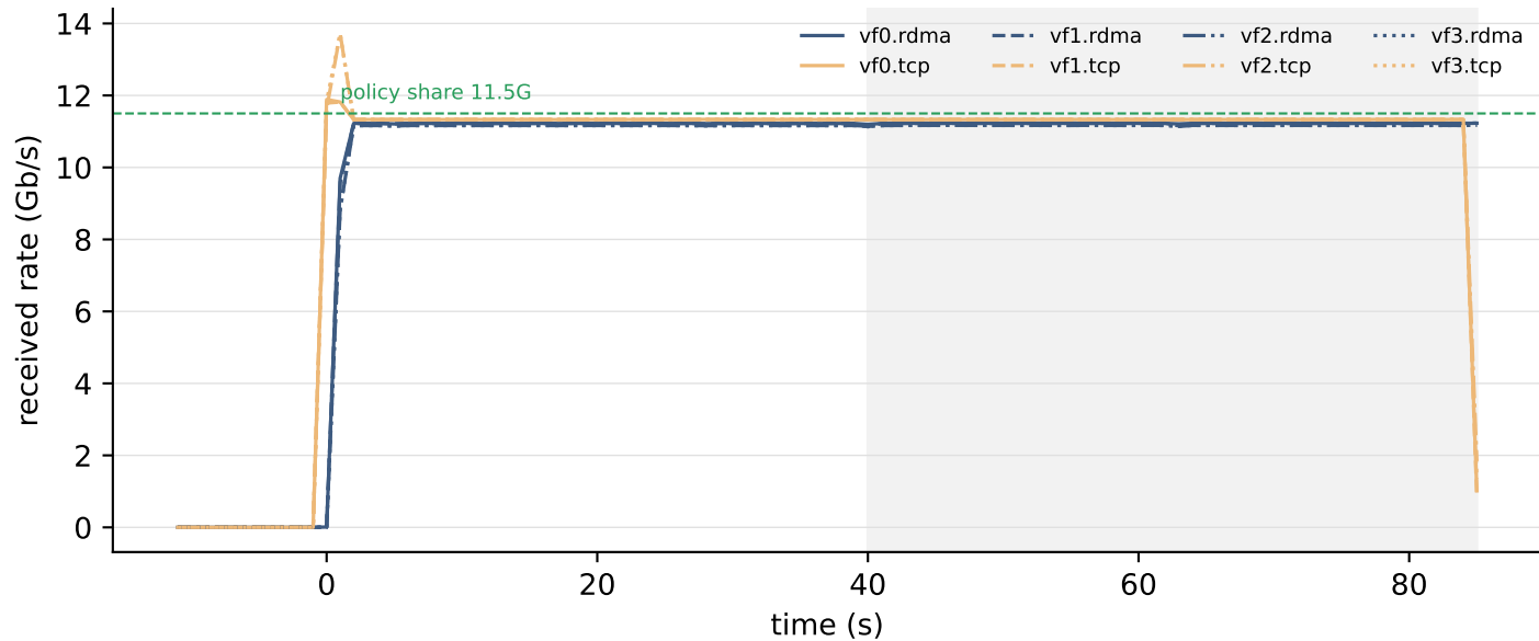
incast8 — DCQCN, coupled recovery, run 2
