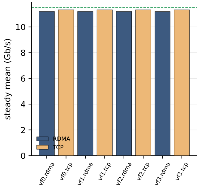
Jain=1.000 agg=90G
