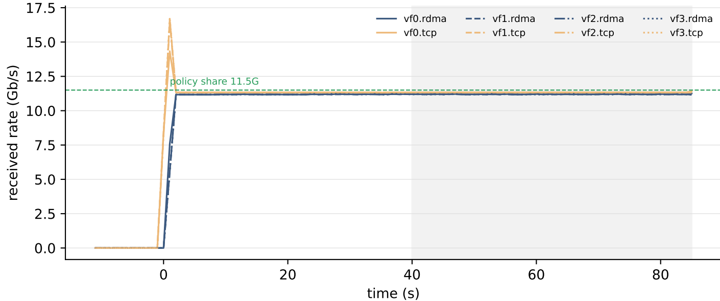
incast8 — observer, DCQCN untouched, run 1
