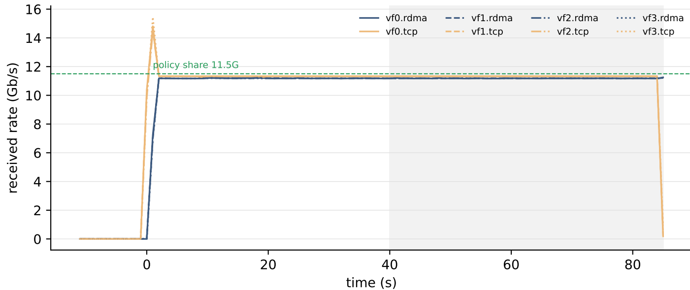
incast8 — observer, DCQCN untouched, run 2
