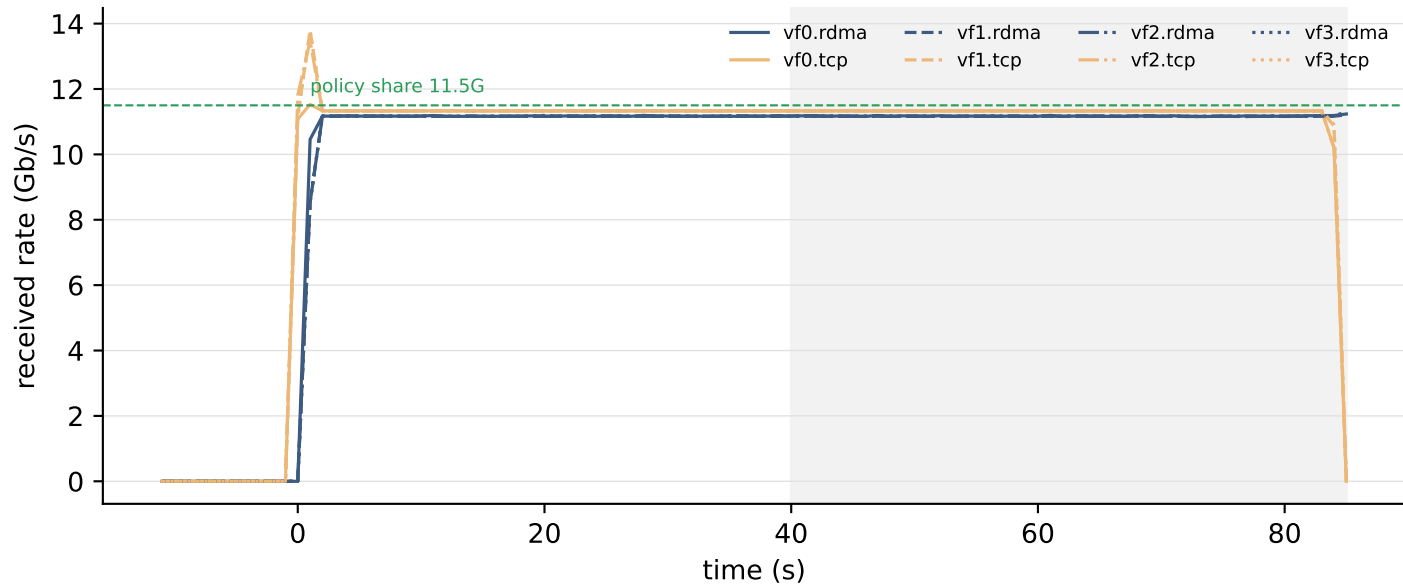
incast8 — observer, DCQCN untouched, run 3
